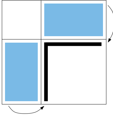
Figure 1: The computational pattern for the Crout factorization. The dark area shows the parts of the factors being computed at the k -th step. The shaded areas show the parts of the factors being accessed at the k -th step.
