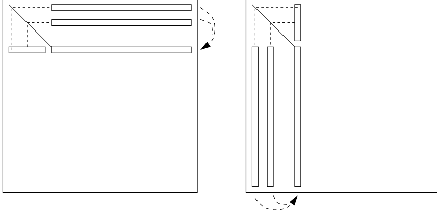
Figure 2: Construction of the k -th row of U (left side) and the k -column of L (right side).
