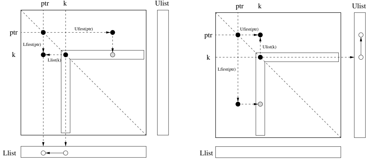
Figure 3: Procedure for updating row k of U and column k of L .
