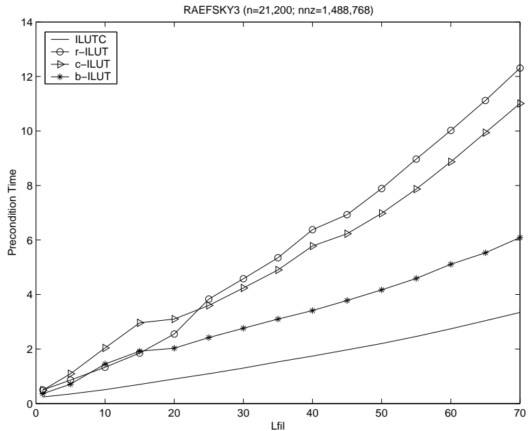
Figure 4: Precondition time vs. Lfil for ILUC, r-ILUT, c-ILUT and b-ILUT ( \tau = 0.001 )
