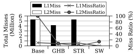
Fig. 26. # Cache misses ratio in 462.libquantum.
