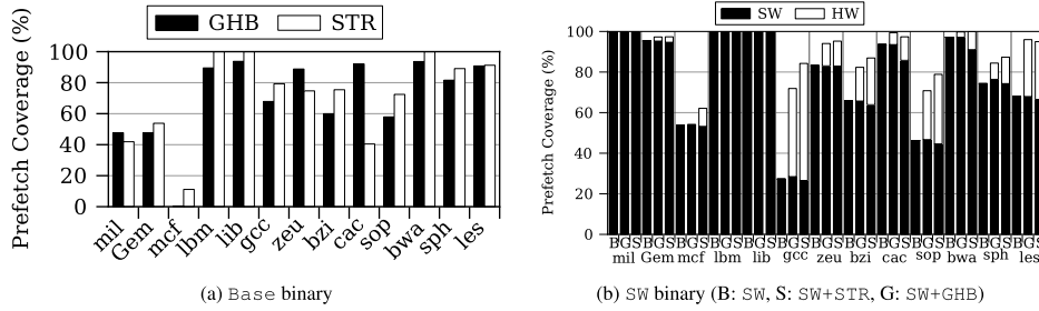
Fig. 10. Prefetch coverage.
