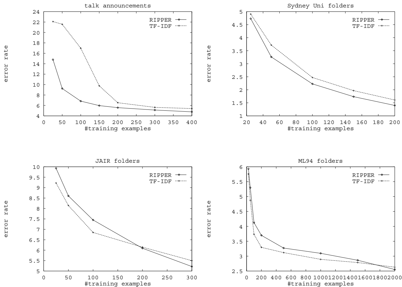
Figure 2: Error rates for various problems
