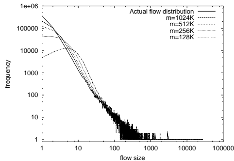
Figure 3: The distribution of flow sizes and raw counter values using varies number of counters (both x and y axes are in log-scale). m = number of counters.
