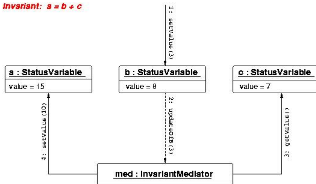
Figure 6: Mediated Invariant Maintenance
