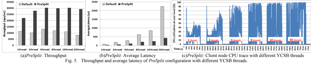
Fig. 5. Throughput and average latency of PreSplit configuration with different YCSB threads.
