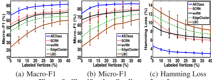
Figure 8: Classification Quality on Last.fm
