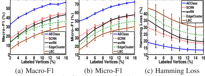
Figure 9: Classification Quality on IMDb
