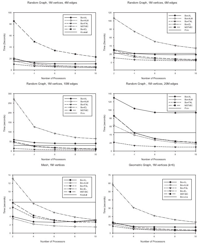
Figure 4. Comparison of parallel MST algorithms for random graph with n = 1M vertices and m = 4M, 6M, 10M , and 20M , edges; for a regular mesh with n = 1M vertices and for a geometric graph with fixed degree k = 6 .
