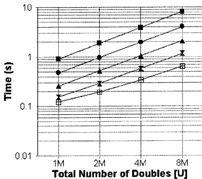
Scalability in Machine & Problem Size on the SP-2-WN
