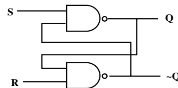
B. SR Latch Diagram
