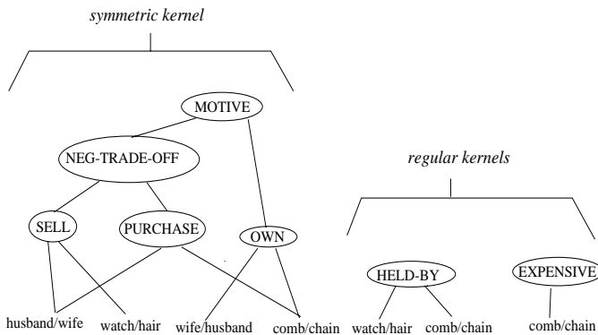
Figure 3 Mapping kernels from Figure 1(c).
