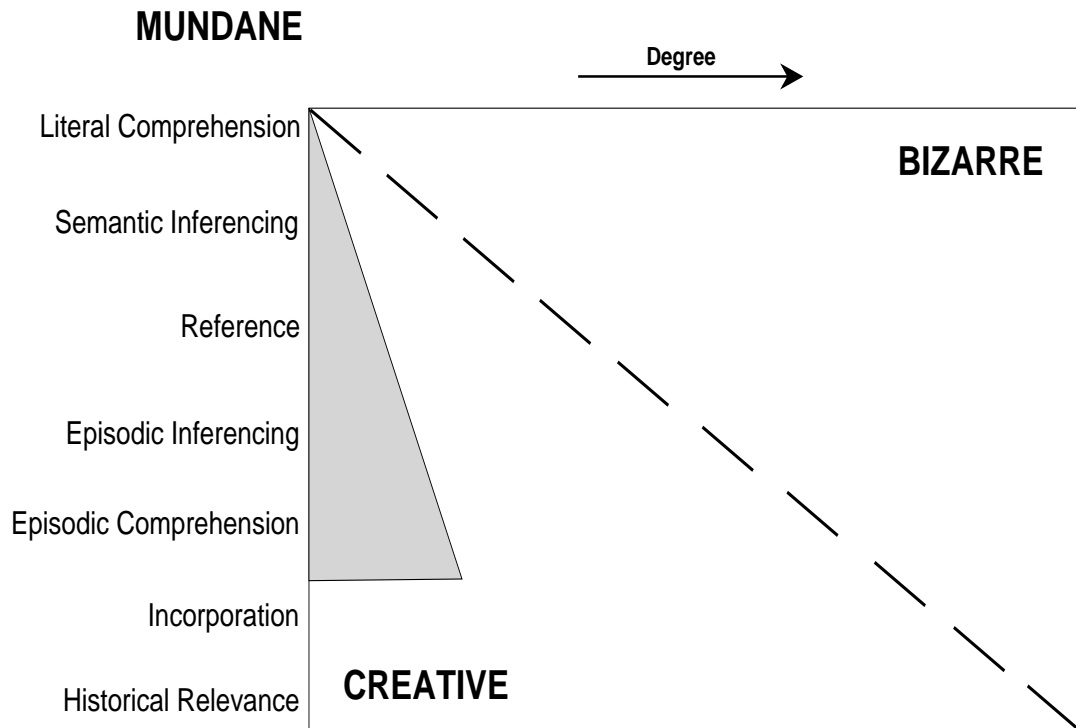
Figure 8: Evaluation
