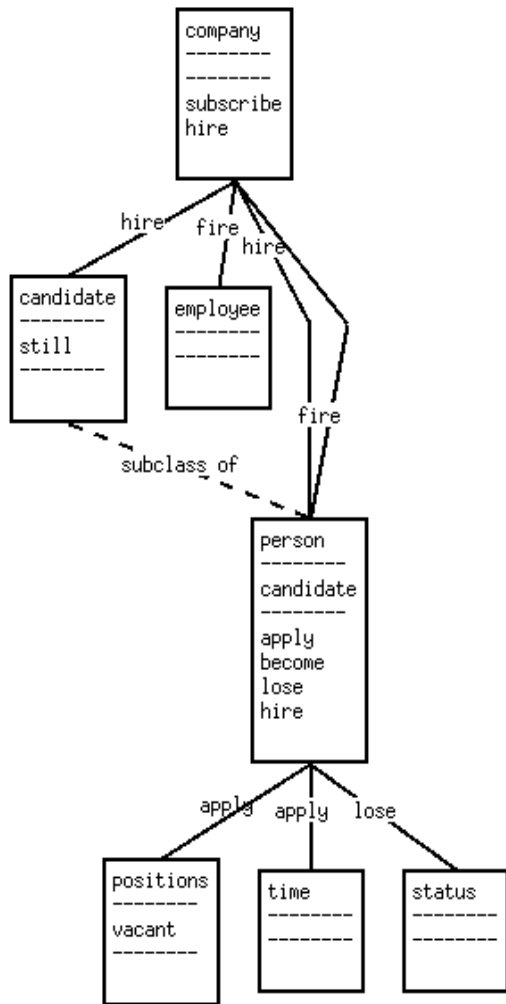
Figure 1: Object Diagram for Employment Database Example
