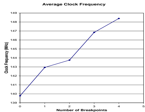
Figure 11: Average clock frequencies.
