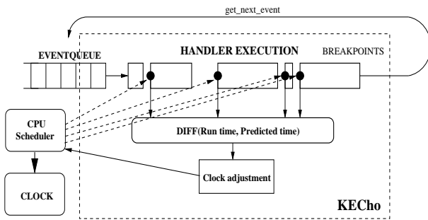
Figure 12: Scheduler breakpoints.
