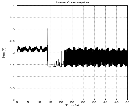
Figure 5: Power consumption without adaptive frequency selection.
