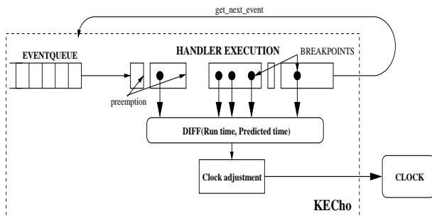
Figure 9: Handler breakpoints.
