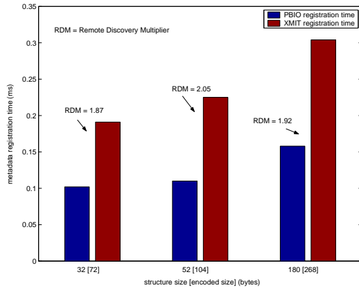
Figure 3. Format registration costs using PBIO and XMIT.
