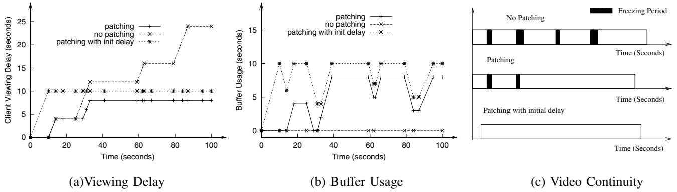
Fig. 12. Video patching on client video reception
