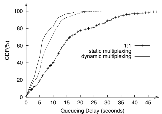
Fig. 17. Client Requests Queuing Delay
