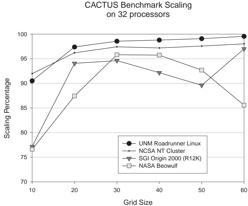
Figure 12: CACTUS scalability.
