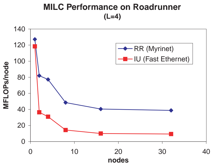
Figure 8: MILC Benchmark with L = 4 .
