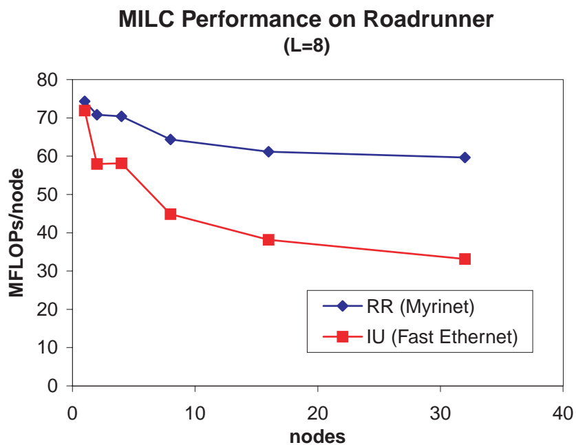
Figure 9: MILC Benchmark with L = 8 .
