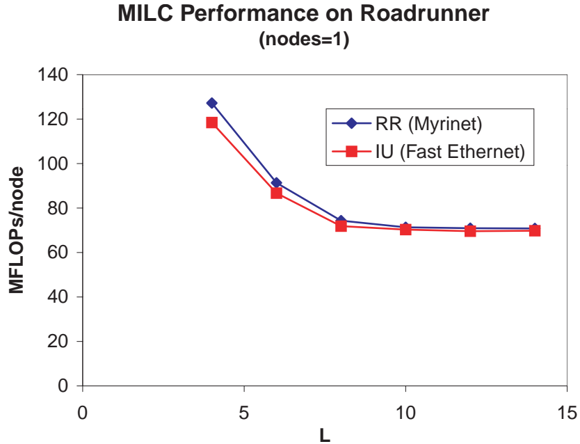
Figure 7: MILC single node benchmark.
