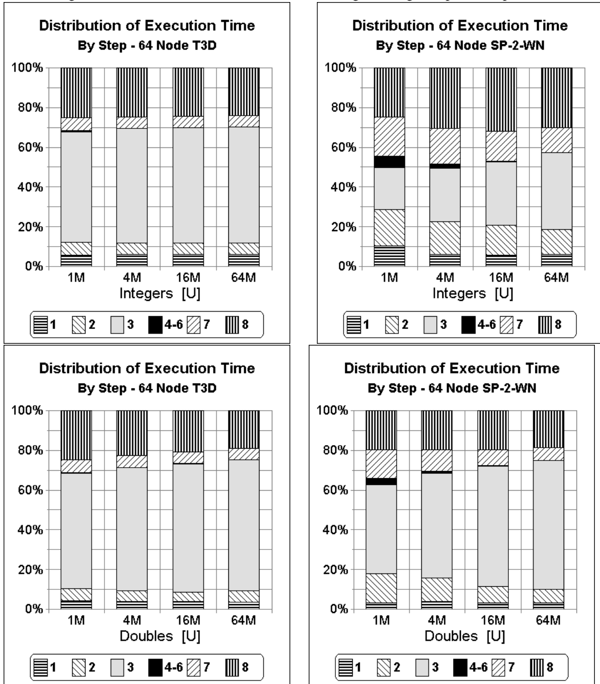
Figure 3: Distribution of the execution time amongst the eight steps of sample sort.
