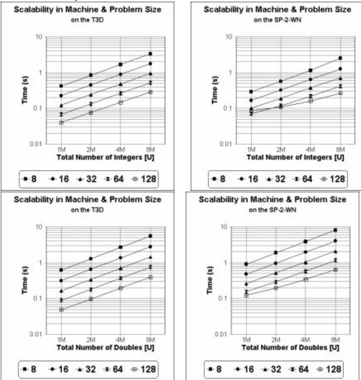
Figure 2: Scalability of sorting integers and doubles with respect to the problem size, for differing numbers of processors.
