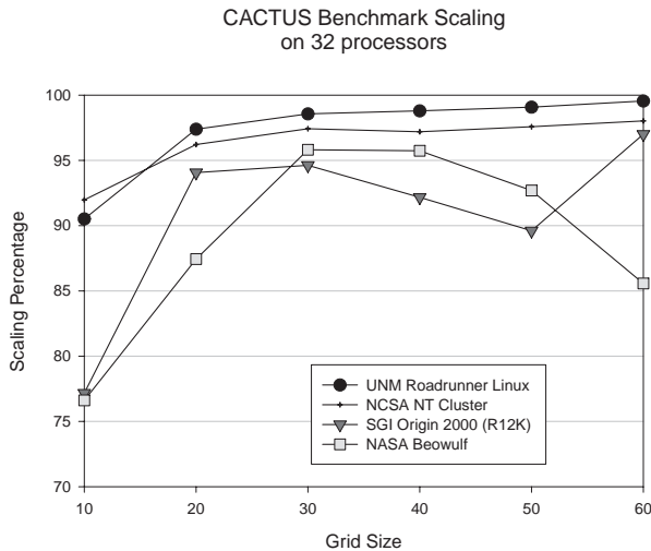
Figure 12. CACTUS scalability.
