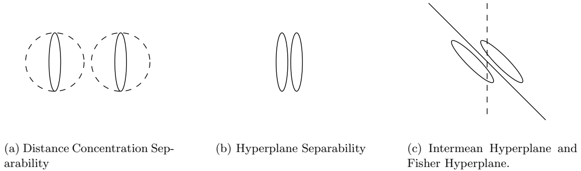
Figure 2: Previous work requires distance concentration separability which depends on the maximum directional variance (a). Our results require only hyperplane separability, which depends only on the variance in the separating direction(b). For non-isotropic mixtures the best separating direction may not be between the means of the components(c).
