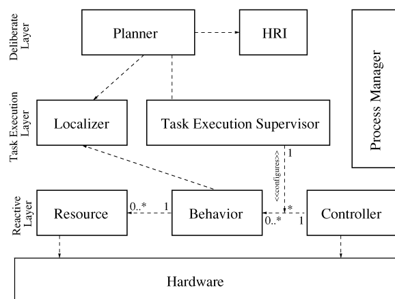
Figure 6. A UML model of the implemented architecture.
