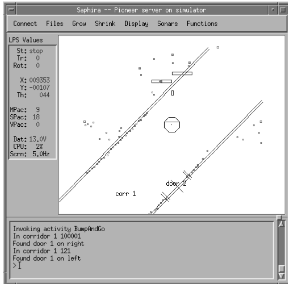
Figure 7. The Saphira graphical user interface.
