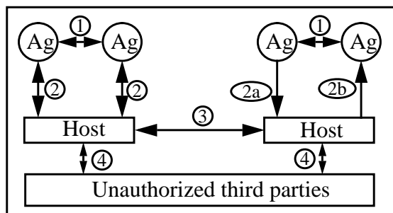
Figure 16: Security Areas of Mobile Agent Systems
