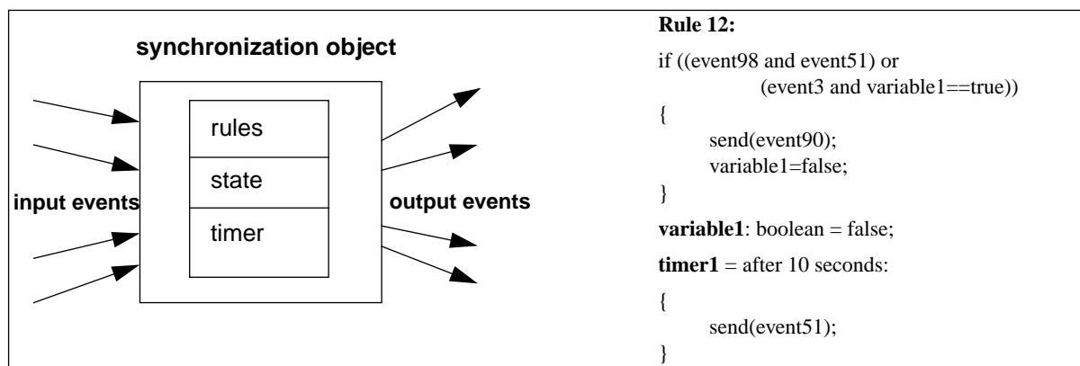
Figure 11: Synchronization Object
