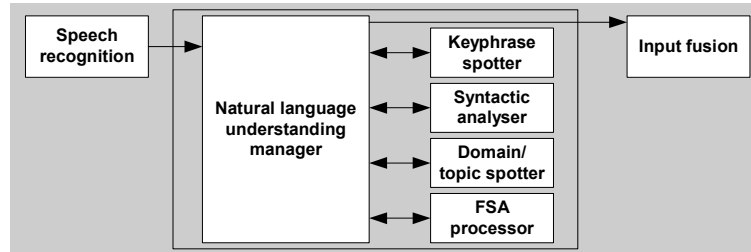
Figure 2. NICE HCA natural language understanding module.
