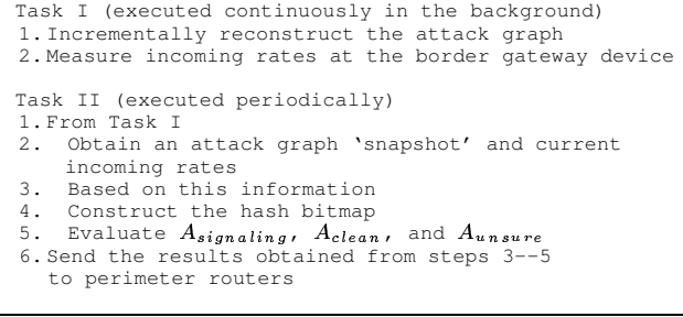
Figure 6. Attack Mitigation Decision-making (AMD) algorithm
