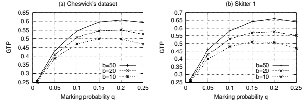
Figure 11. GTP (Good traffic Percentage) by varying parameter b
