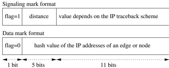
Figure 4. Mark format for signaling and data subchannels
