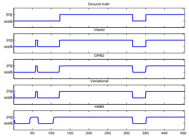
(b) Four switching state models, first order SLDS.
