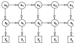
Figure 1. Bayesian network representation (dependency graph) of the SLDS. s denote instances of the discrete valued action states switching the physical system models with continuous valued states x and observations y .
