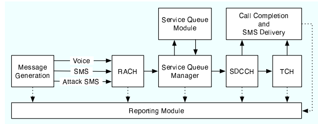
Figure 18: Simulator Architecture
