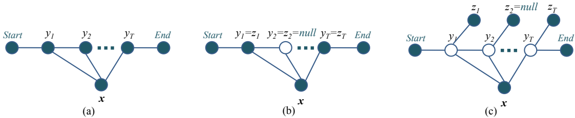
Figure 1: Graphical model representation of CRFs for three different training settings: (a) supervised CRF; (b) semi-supervised CRF with derived labels as hard evidence; (c) semi-supervised CRF with derived labels as soft evidence. Solid and empty nodes denote observed and hidden variables respectively.
