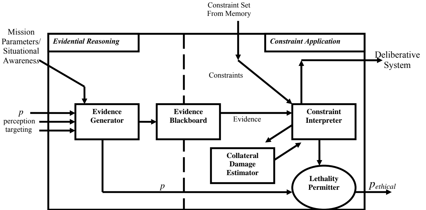
Figure 3. Architecture and data flow overview of the prototype ethical governor
