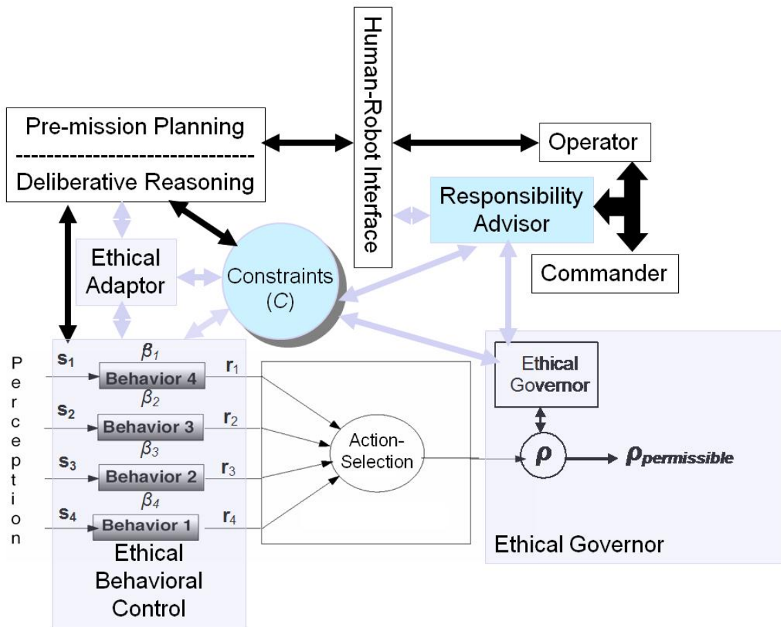
Figure 6: High level schematic of the ethical hybrid-deliberative reactive architecture. The newly developed ethical components are shown in color. The ethical governor is discussed in Section 2 and the ethical adaptor in Section 3 of this article. Details of the ethical behavioral control and the responsibility advisor components are presented elsewhere [Arkin 09, Arkin et al 09].
