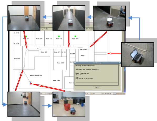
Figure 2: Biohazard Search
