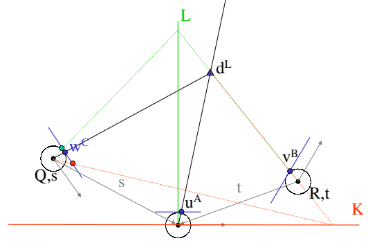
Figure 5: Intrinsic homographies K and L , see text.
