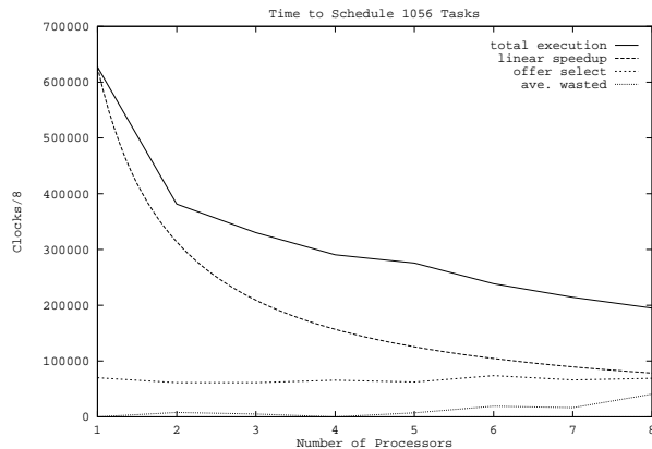
Fig. 5. Multiprocessor Performance
