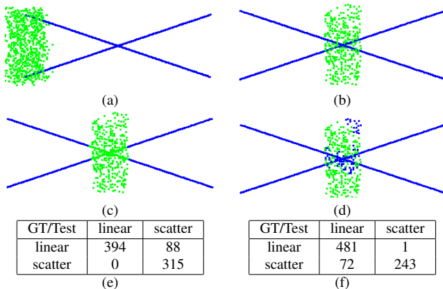
Figure 3. Difference between directional features and directional potentials, with the lines/scatter points in blue/green. (a) Training data. (b) Ground truth for the testing data. (c) Standard AMN. (d) Directional AMN. (e)/(f) Confusion matrix for standard/Directional AMN.
