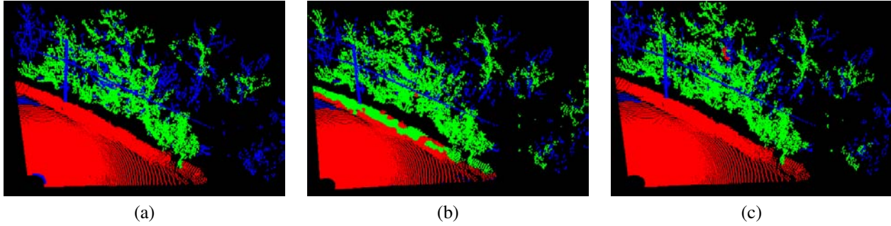
Figure 5. Classification results on "sweeping" data set for three labels (linear/scatter/surface). (a) AMN classification. (b) Directional AMN (linear, surface) classification. (c) Directional AMN (linear) classification.
