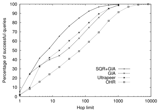
Fig. 9. Success rate of queries vs. hop limit in a network with replication according to the Zipf distribution. Notice the contrast with figure 6(b).
