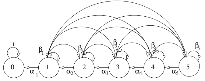
Fig. 4. A Markov chain model of routing using SQR.
