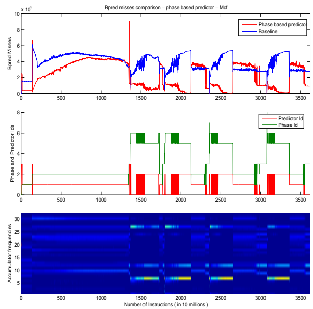
Figure 5: Branch predictor misses comparison for mcf. This graph provides a comparison of branch predictor misses in the phase-based branch predictor scheme with those in the baseline case for the mcf benchmark. The second part of the graph shows the phases predicted by the phase predictor and the corresponding branch predictor chosen for that phase. The third part of the graph shows the scaled values of the accumulators used in the phase tracking scheme.
