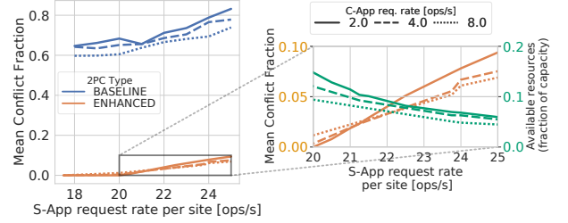
Figure 6: MCF of baseline and enhanced 2PC for typical S -App and C -App request rates from the SF cabs dataset (Table 2). The blow-up shows the increase in MCF and the \mu DC’s remaining available resources for enhanced 2PC.
