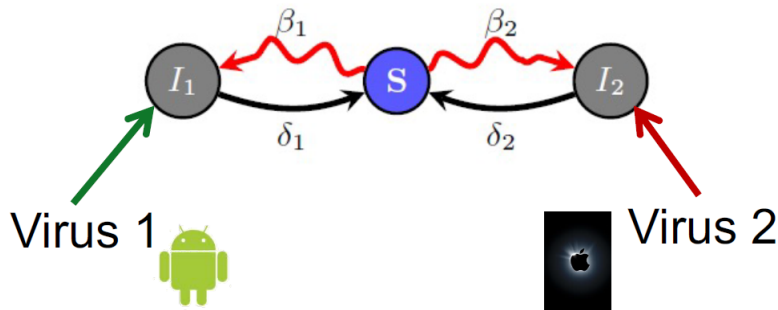
Figure 6: A two-contagion model diagram. Image from Slide 38 of Lecture 5
