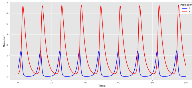
Figure 5: Example Lotka-Volterra model.
