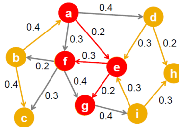
Figure 3: Example IC model diagram with the individual edge weights. Image from Slide 4 of Lecture 5
