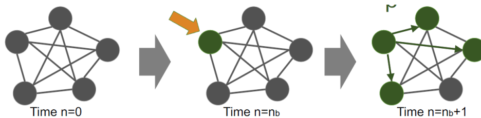
Figure 4: Example SpikeM model diagram. Image from Slide 12 of Lecture 5
