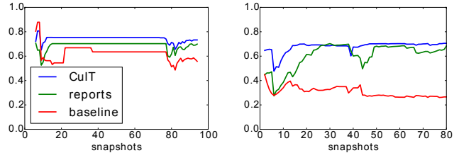
Figure 7: MCC on Flixster (left) and Enron (right).
