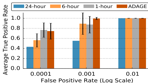
Figure 3: Detecting malicious files/machines via belief propagation on Symantec edge streams. ADAGE intervals have the best performance.
