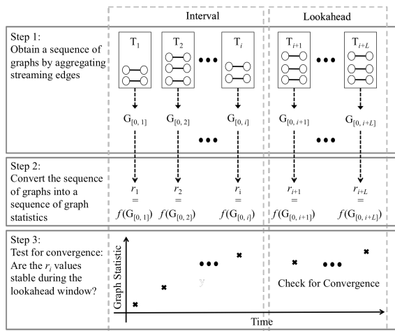
Figure 2: ADAGE Overview: Edges are aggregated until convergence is detected on the chosen statistic.
