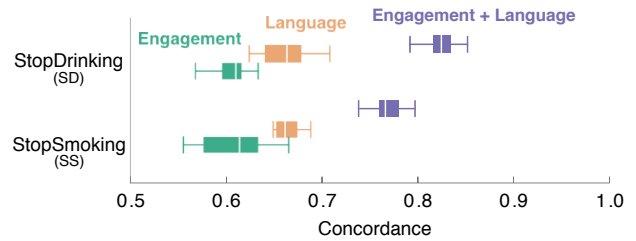
Figure 5: Boxplots for 10-fold cross-validated concordance scores of the statistical models. The ENGAGEMENT + LANGUAGE model gives significant predictive power with a mean concordance of 0.77 in StopSmoking (SS) and 0.82 in StopDrinking (SD).
