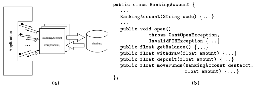
Fig. 1. (a) High-level view of the application. (b) Interface of the BankingAccount component.
