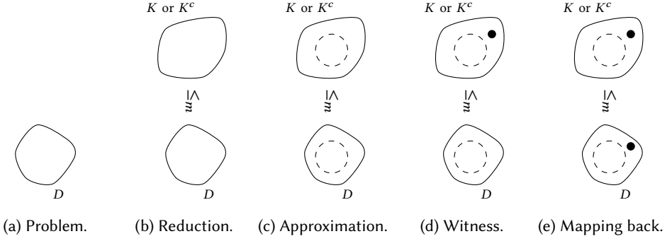
Fig. 4. Construction overview: (a) constructing a decision problem D , (b) constructing a many-one reduction \leq_m from K to D , (c) constructing an approximation for K (the dashed circle in K ) based on the approximation for D (the dashed circle in D ), (d) constructing a witness in K (the black point in K ), (e) mapping the witness in K back to a witness in D (the black point in D ).
