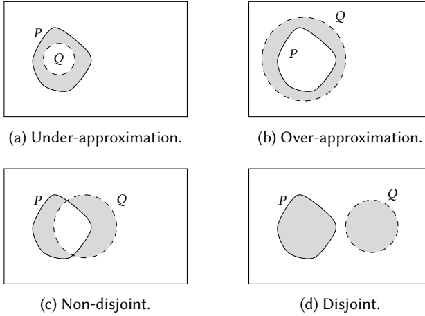
Fig. 1. Four cases of an undecidable problem P and its decidable approximation Q . The grey areas ( P\Delta Q ) represent the imprecision. The trivial case of Q = \emptyset could be classified as either case (a) or case (d). The rectangle surrounding each case represents the set of all natural numbers.
