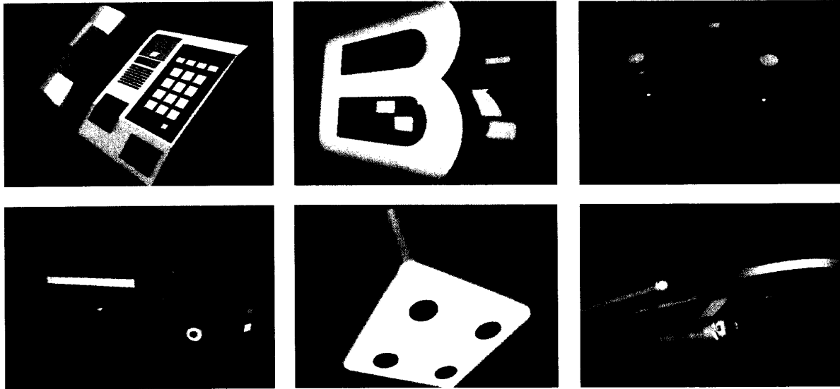
Figure 7. Images generated with the Pixel-planes 4 solid modeler.
