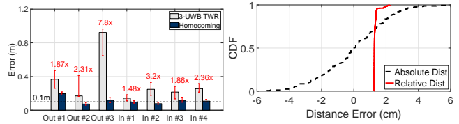
Figure 5: (a) Overall localization errors of Homecoming. (b) Comparison of distance measurement stability using time of flight and relative phase differences.
